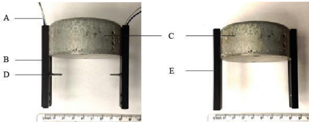
(a) A. Wires (+/-). B. Delrin® slide bars with BE. D. Bender element. (b) C. Aluminum loading cap. E. Delrin® slide bar without BE.
