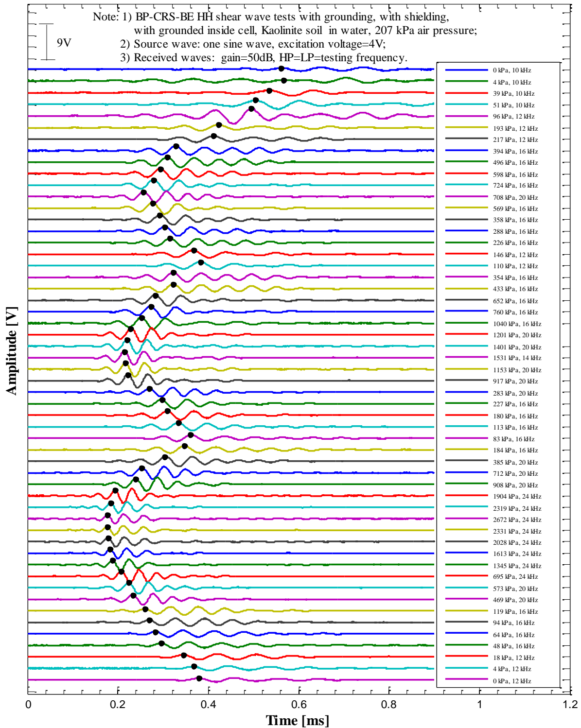
Figure B.8. Waterfall plot of collected shear wave signals of BP-CRS-BE T10 tests on kaolinite soil for determination of V_s (HH) during consolidation tests (oscilloscope collected shear wave signals, test date: 12/07/2015).
