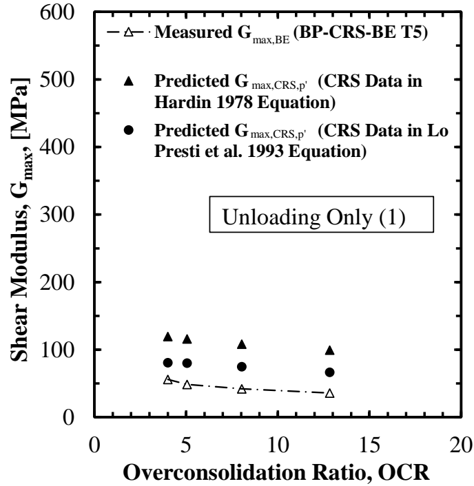
Figure C.17. Shear modulus as a function of overconsolidation ratio for BP-CRS-BE T5 on Kaolinite soil specimen (unloading 1).
