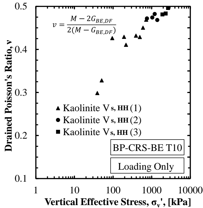
Figure C.54. Poisson's ratio as a function of vertical effective stress for BP-CRS-BE T10 on Kaolinite soil specimen (loading only).
