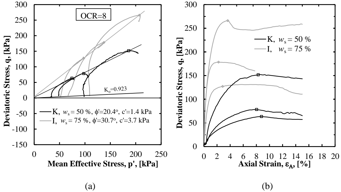
Figure 6.18. Comparison of the behavior of the 50-percent Kaolinite and 75-percent Illite samples as conducted in triaxial tests in terms of: (a) deviatoric stress as a function of mean effective stress, and (b) deviatoric stress as a function of axial strain.
