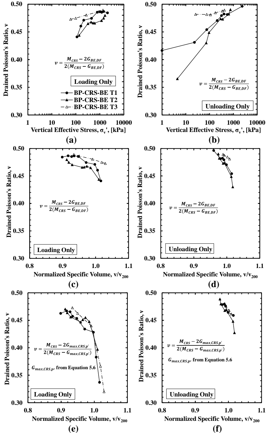
Figure 5.14. BP-CRS-BE testing results of Poisson's ratio-verticial effective stress relationship for (a) loading stage, (b) unloading stage; measured Poisson's ratio-normalized specific volume relationship for (c) loading stage and (d) unloading stage; and predicted Poisson's ratio-normalized specific volume relationship for (e) loading stage and (f) unloading stage.
